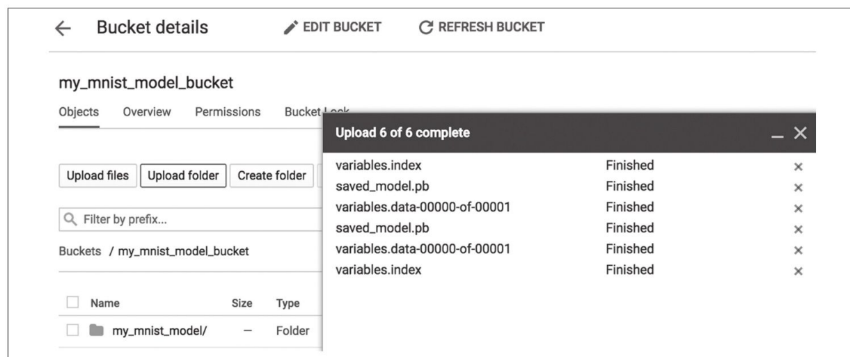
图19-4：将SavedModel上传到Google Cloud Storage
