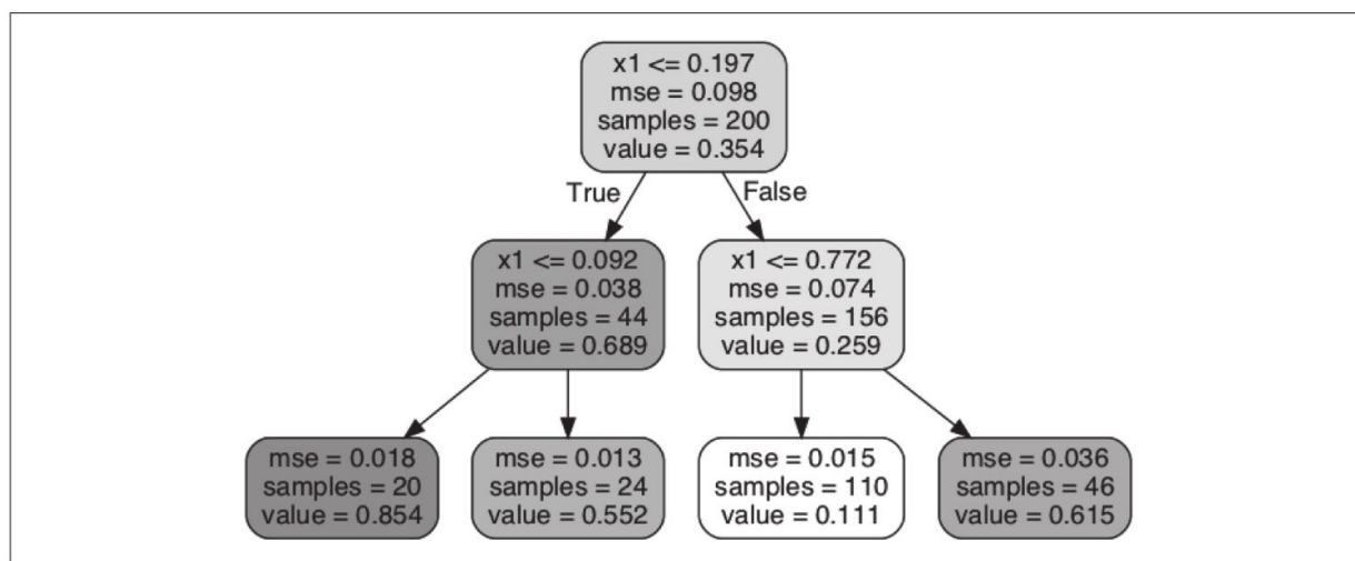
图6-4：回归决策树
